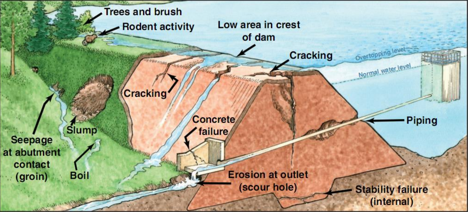
Some causes of dam failures
